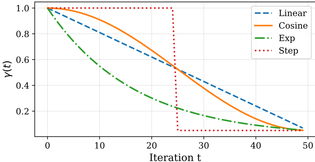
Diversity Coefficient \gamma(t) Schedules
